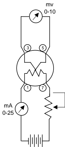
TYPICAL CIRCUIT
