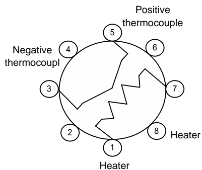
BASING DIAGRAM
