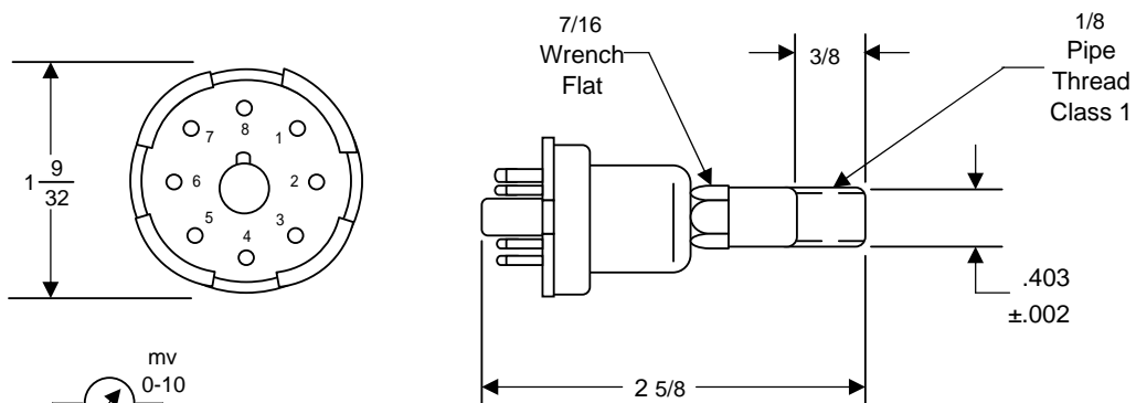
OUTLINE DRAWING
